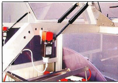
Safety switches on doors, if opened machine stops.
