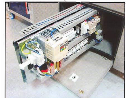
Control Panel slides out for easy access to all electrical components.
