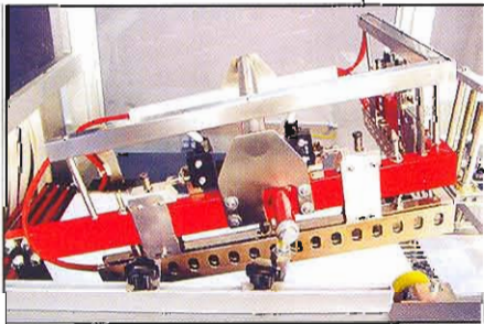
Single piece hot knife seal bar with round corner cut off.
