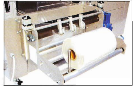
Powered film unwind with easy load film cradle and pin wheel hole punch.
